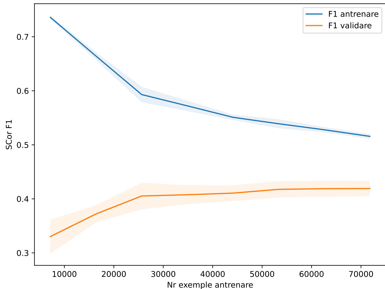
Curba invatare - Random Forest
